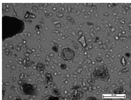
31. ábra PA11 20-25 cm minta: globular psilate morfortípus Figure 31. Globular psilate morphotype from sample PA11 20-25 cm
