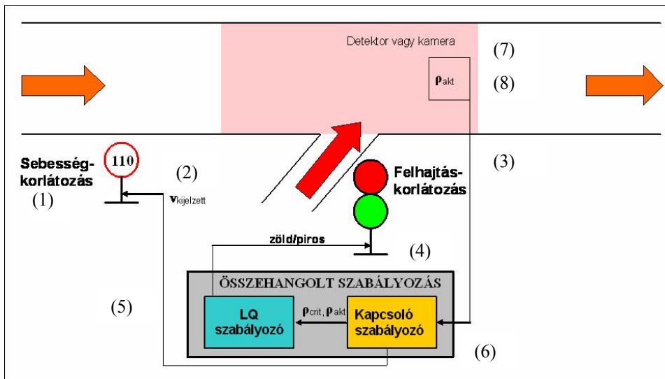
Figure 5. The controlled freeway stretch
