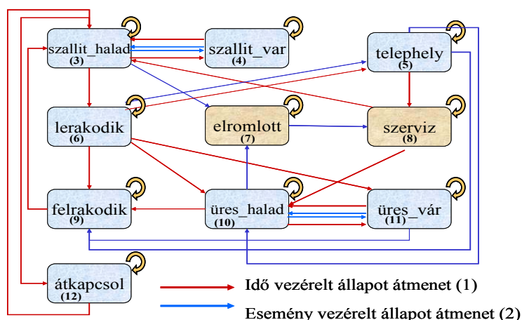
Figure 3: Possible States and Transitions
