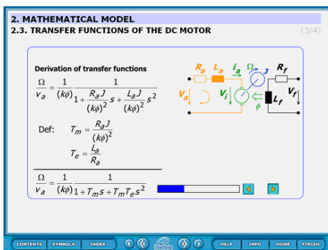
Figure 3: Transfer function
