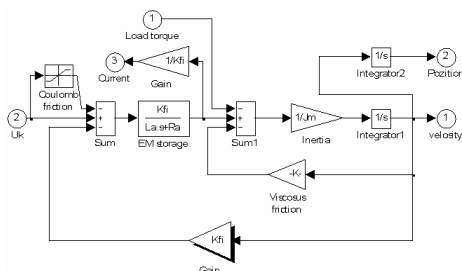
Figure 7: Model of the DC motor
