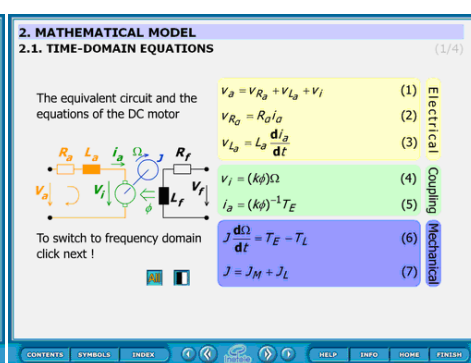
Figure 2: Time-domain equations
