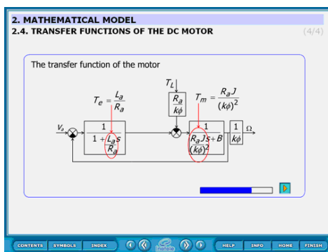
Figure 4: Block diagram
