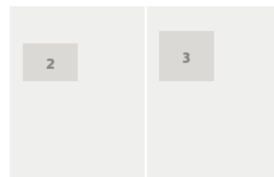
Fig. 2: Rokström-Shudev: Pyramid of SDGs (2014) (SOURCE: HTTPS://ECOACSA.COM/EN/SDG/ )
